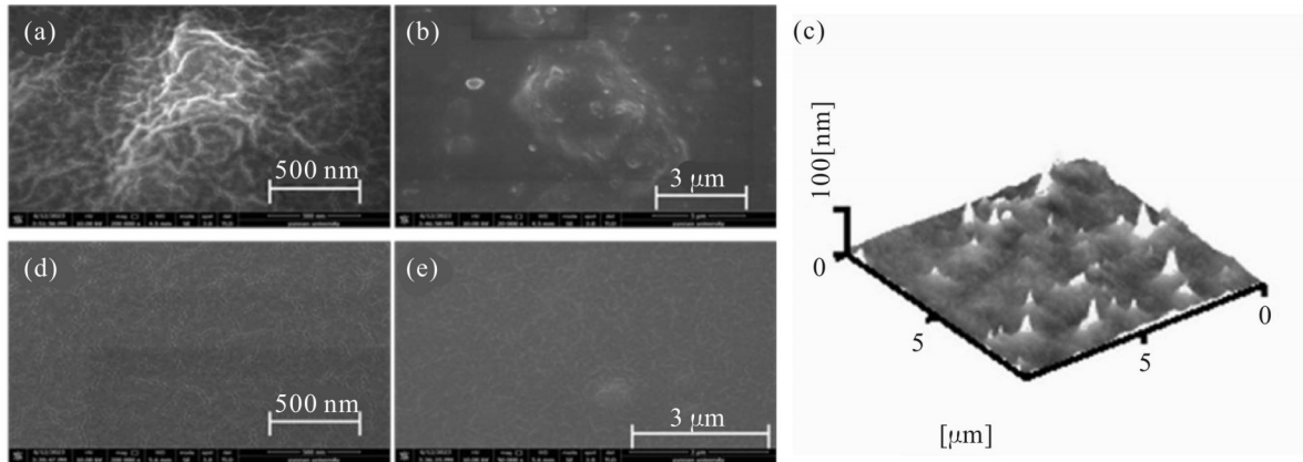
Fig. 2 Surface morphologies of coating: (a, b) SEM images of Brush preparation super smooth coating; (c) AFM images of super smooth coating; (d, e) SEM images of Dip preparation super smooth coating
