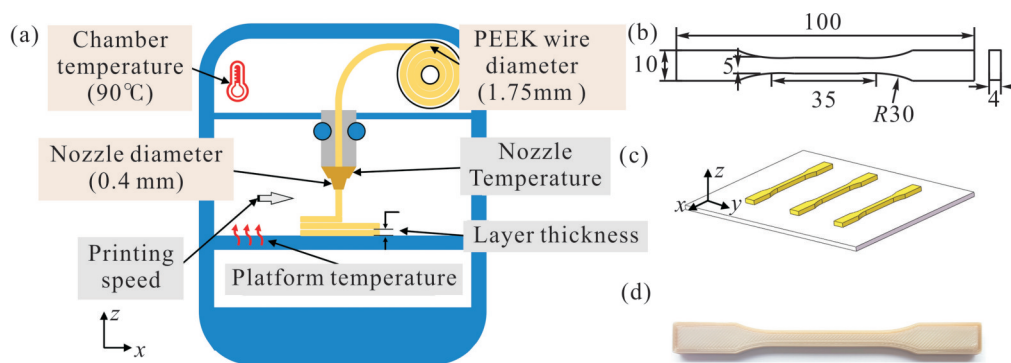
Fig. 1 FDM printing of PEEK samples: (a) schematic of FDM printed PEEK sample; (b) design dimensions of PEEK sample; (c) printing direction and quantity; (d) FDM printed PEEK sample
