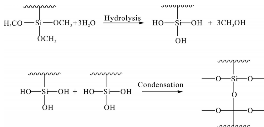
Scheme 1 Crosslinking reaction of A-171
