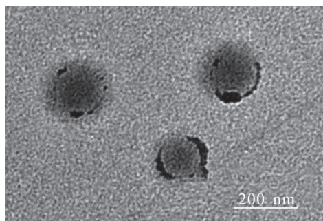
Fig. 4 TEM image of core-shell acrylic emulsion
