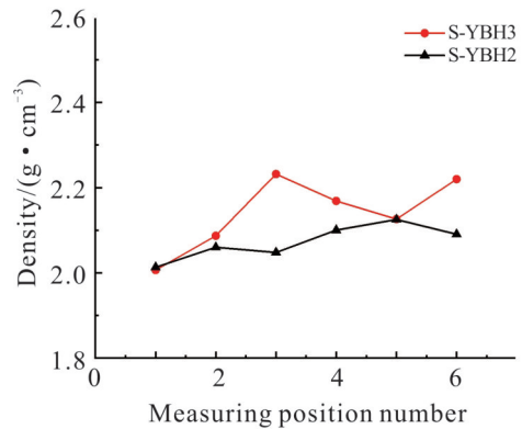
Fig. 7 Density of PTFE membrane after heat treatment
