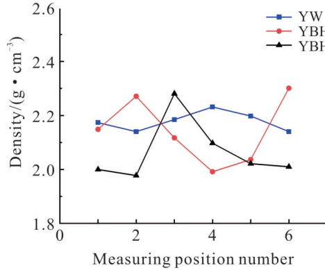
Fig. 6 Density of original PTFE turning film
