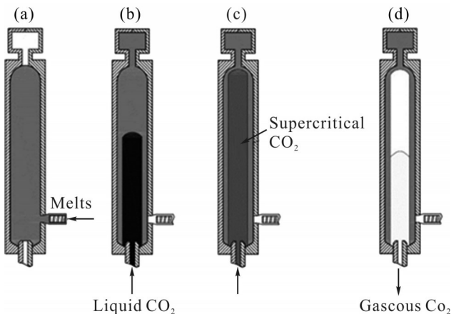
Fig. 3 Schematic diagram of LCO 2 -AIM process
