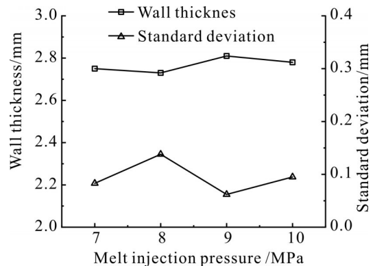
Fig. 9 Effect of melt injection pressure on the wall thickness and uniformity of pipes
