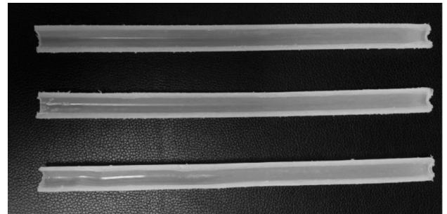
Fig. 6 Each process formed sample and its longitudinal section diagram (from top to bottom are LCO 2 - AIM, GAIM, WAIM, respectively)
