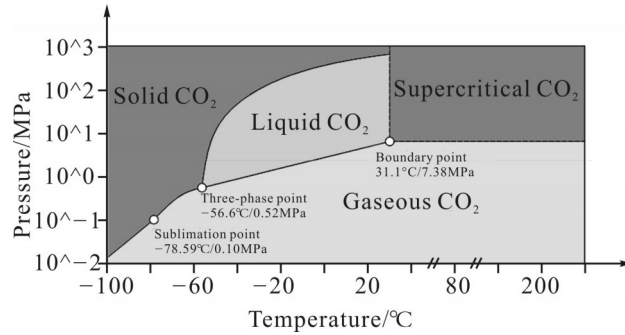
Fig. 1 CO 2 phase transition diagram
