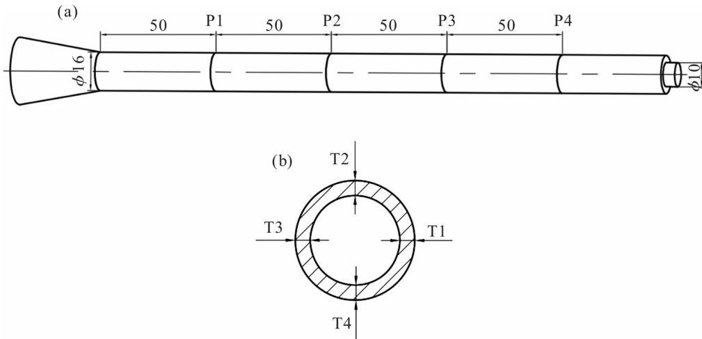
Fig. 5 Residual wall thickness measurement scheme (unit: mm) (a): pipe fitting measurement position; (b): section measurement point
